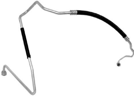
5-9264 FORD: F3DZ-19C836-B Suction Line w/ Accumulator 1993 FORD
