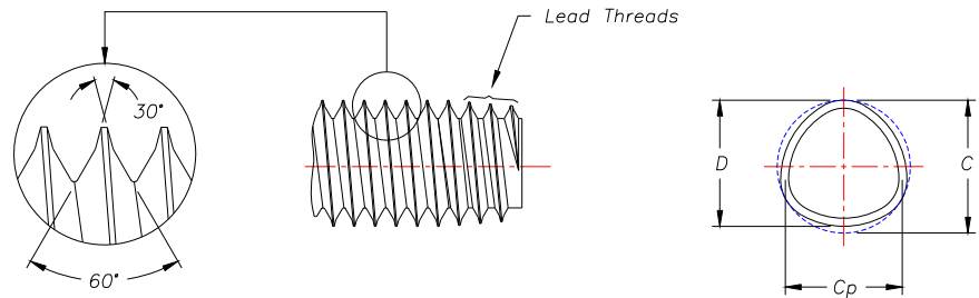
Thread Form Profile
